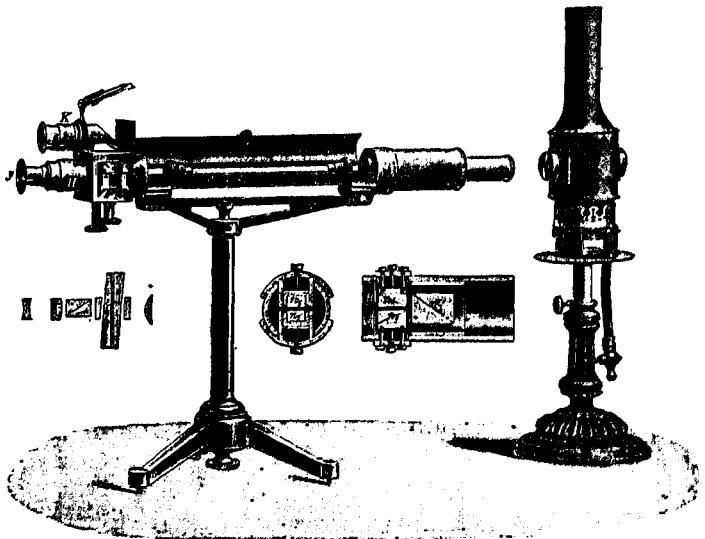
FIG. 21. — DUBILLE-WRIGHT, TRIPLE-SHADE SACHARIMETER WITH DIAGRAM OF OPTICAL PARTS.
