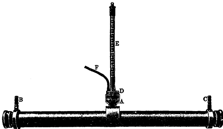
FIG. 23.— WATER-JACKETED TUBE FOR POLARIZING AT CONSTANT TEMPERATURE.
