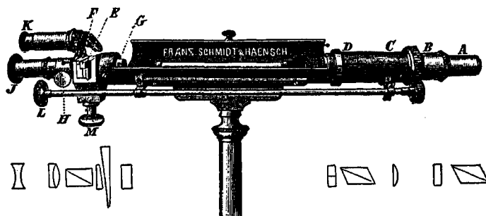
FIG. 22.—SHELL-VRENTZKE-SCHEIBLER TRANSITION-TINT SACCHARIMETER.
