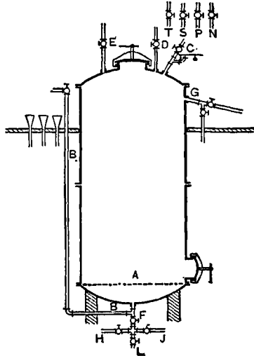
FIG. 37. — SECTION OF BONE-BLACK FILTER.
