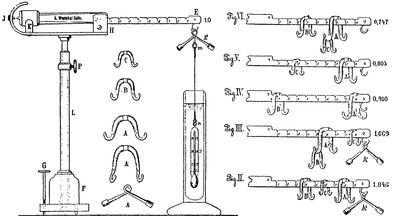
FIG. 30.—DETAIL OF WESTPHAL SPECIFIC GRAVITY BALANCE AND ILLUSTRATION OF MANNER OF READING.
