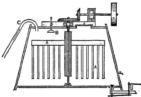
FIG. 36.—SECTION OF NEUTRALIZER.
