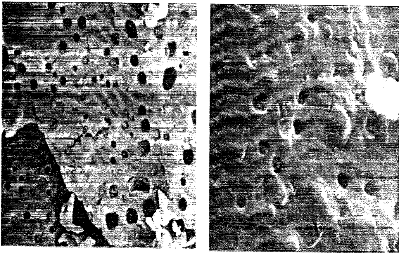
Figure 7. (Left) Composition B (Specimen #2W, 4,200×). (Right) Composition B (Specimen #2F, 10,000×).
