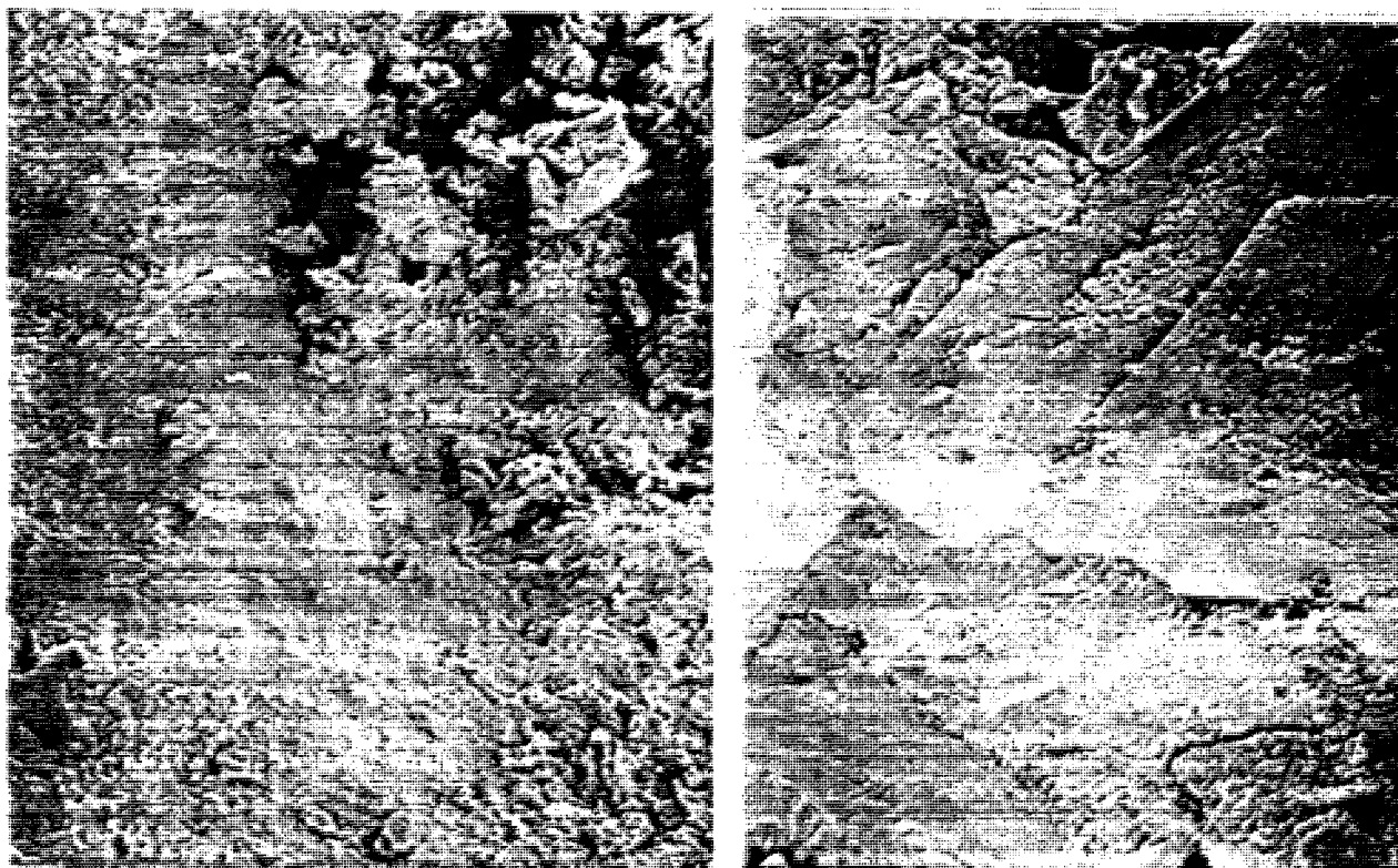
Figure 6. (Left) Weathered PBX 9404 (Specimen #1W, 1,000 \times ). (Right) PBX 9404 fresh cut from weathered piece (Specimen #1F, 1,000 \times ).
