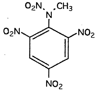
TETRYL FW = 287.1
