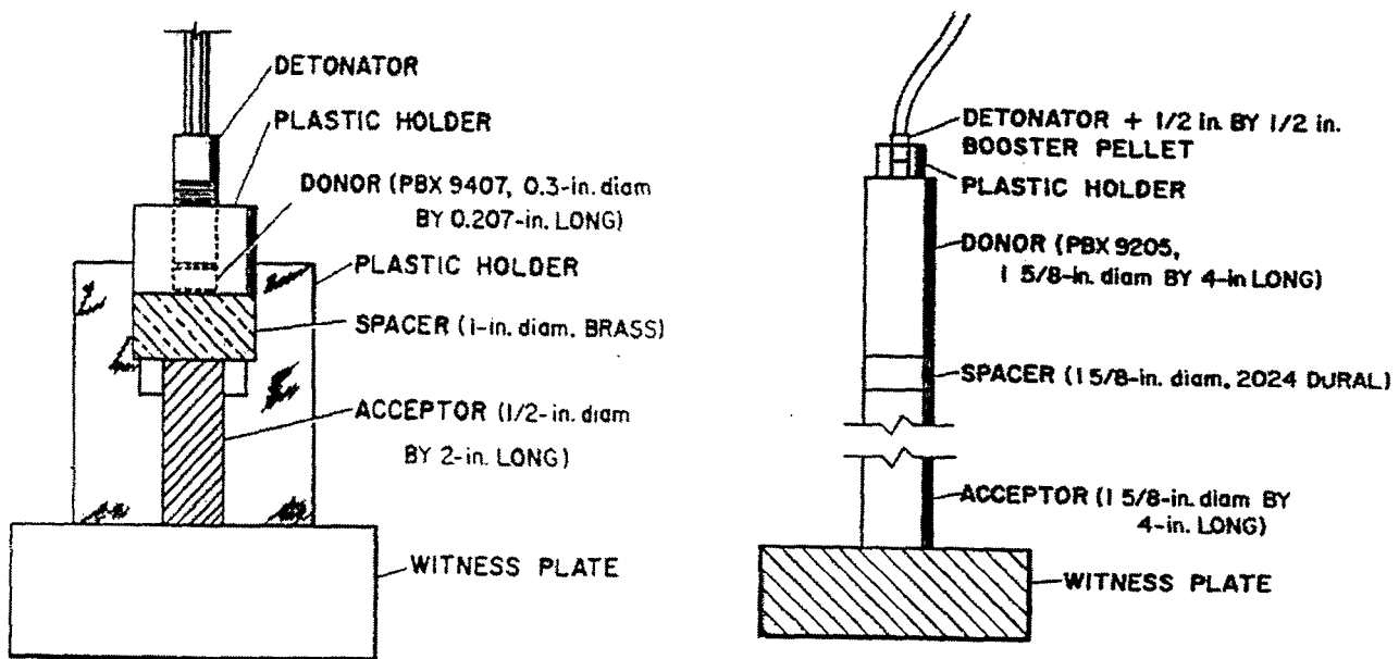
Figure 2. (Left) Small-scale gap-test assembly. (Right) Large-scale gap-test assembly.
