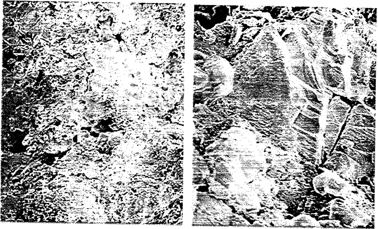
Figure 10. (Left) Inert PBX 900-10 (Specimen #5W, 1,000×). (Right) Inert PBX 900-10 (Specimen #5F, 1,000×).
