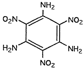
TATB FW = 258.1
