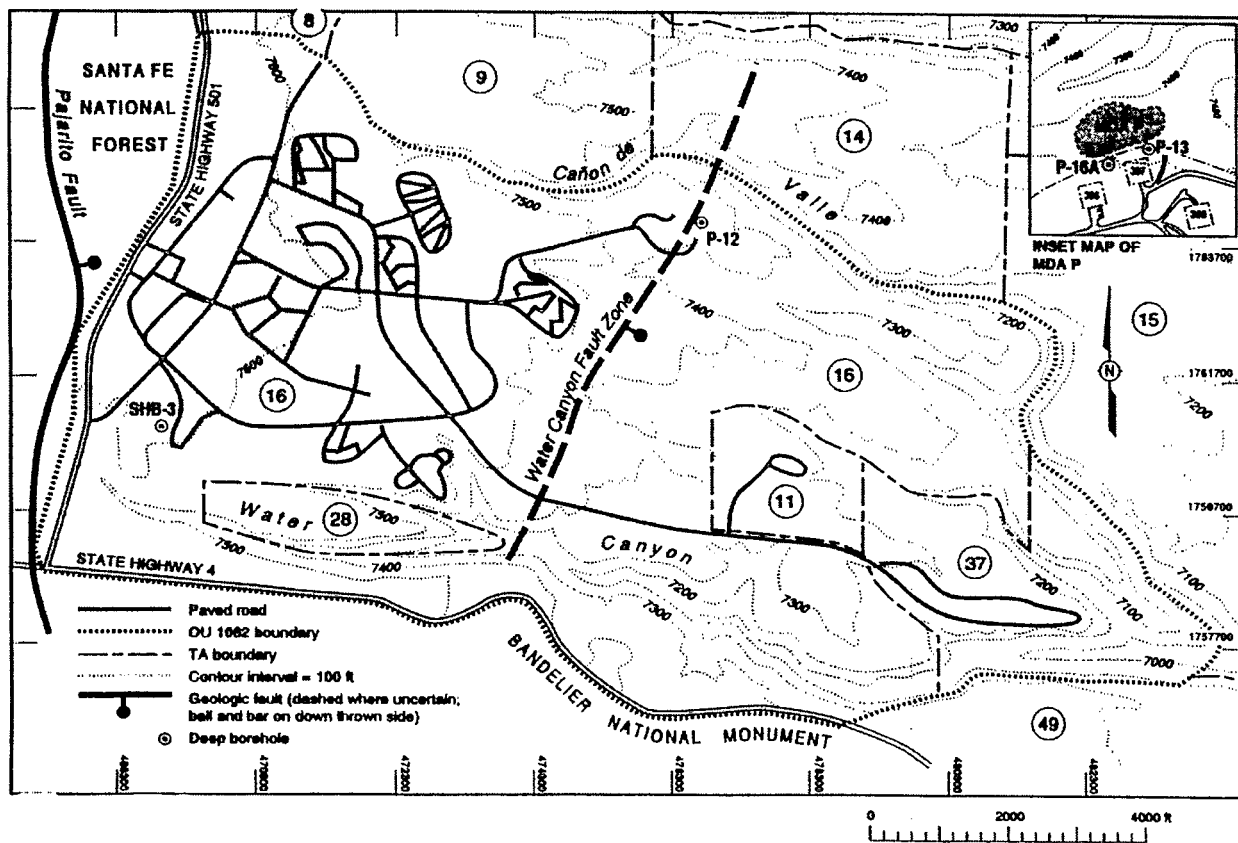
Figure 4. Structural geology and topography of the Weapons Research Area.
