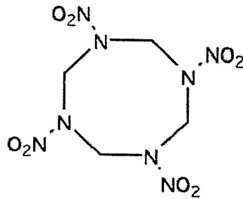
HMX FW = 296.2
