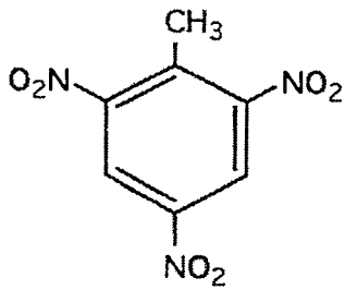
TNT FW = 227.1
