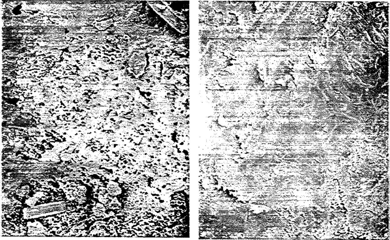
Figure 9. (Left) PBX 9011 (Specimen #4W, 1,000×). (Right) PBX 9011 (Specimen #4F, 1,000×).
