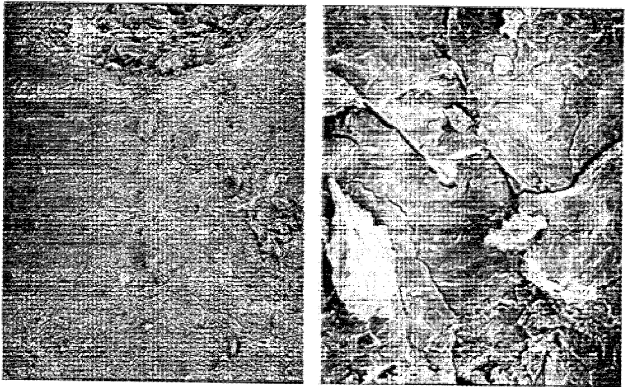
Figure 8. (Left) LX-10 (Specimen #3W, 500×). (Right) LX-10 (Specimen #3F, 1,000×).
