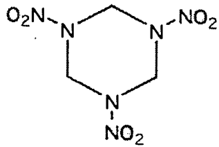
RDX FW = 222.1
