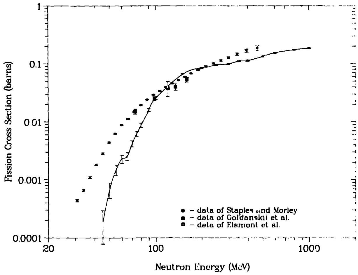
Figure 2: Neutron induced ^{209}\text{Bi} fission cross section. LAHET calculations with Bertini INC and default physics options (line).
