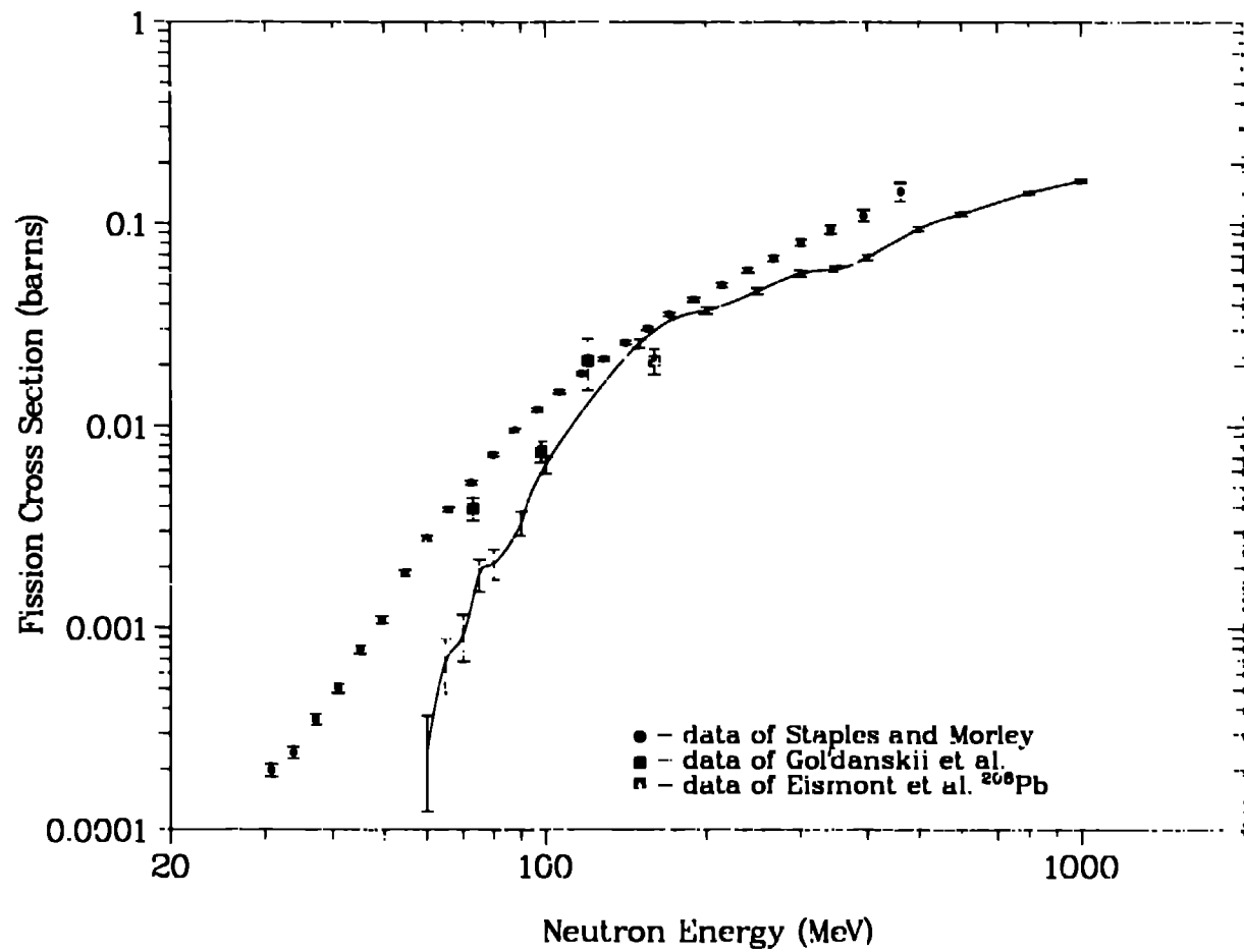
Figure 1: Neutron induced natural Pb fission cross section. LAHET calculations with Bertini INC and default physics options (line).
