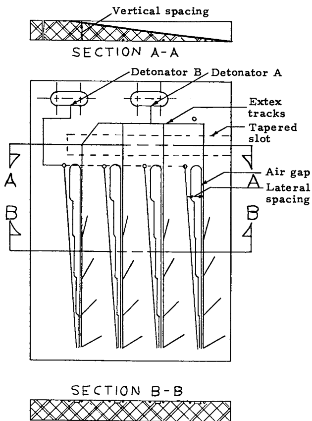
Fig. 9. Sketch of corner turning device.
