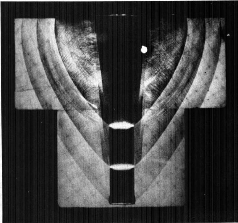
Fig. 3. \text{I}^2\text{C} photograph for Shot C-4632, a 10-cm-diam Plexiglas tube containing ANFO.
